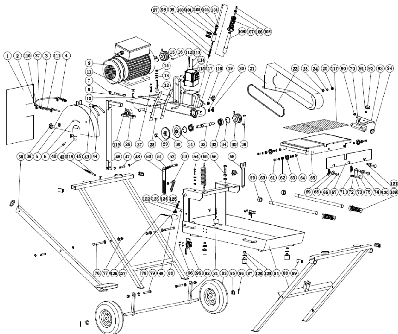
Brick &amp; Masonry Saw (FBS-36E)
