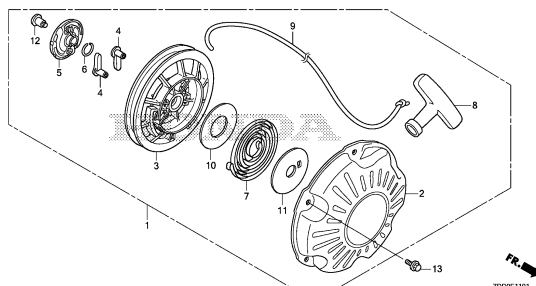
RECOIL STARTER(2)
