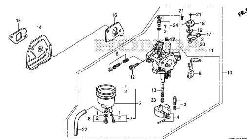
CARBURETOR(STANDARD)
