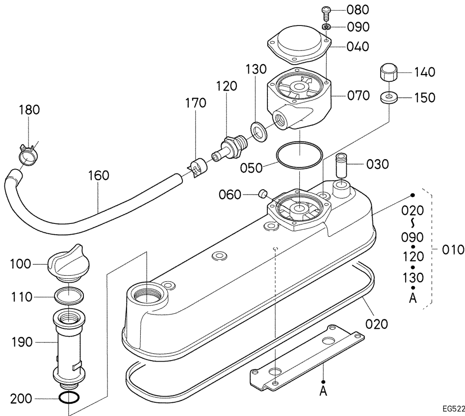
EG522-148-10
