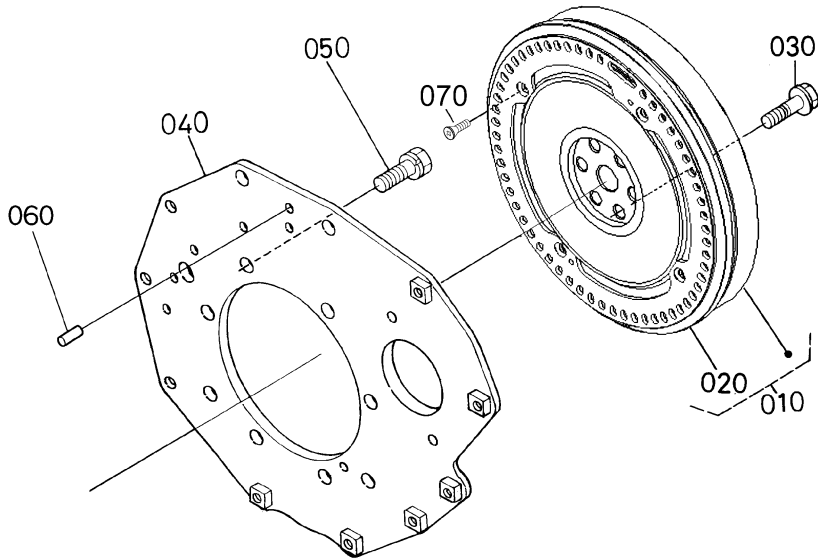
EG525-007-10
