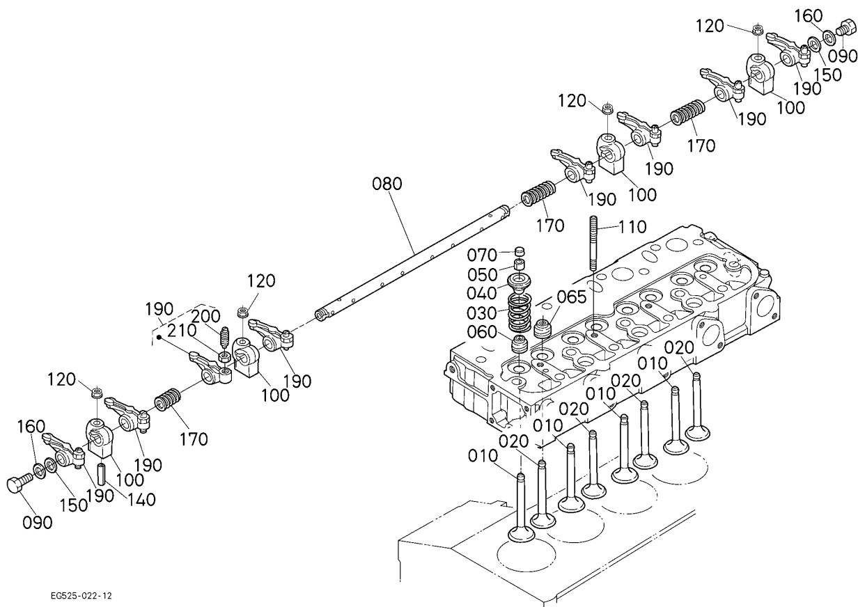
EG525-022-12
