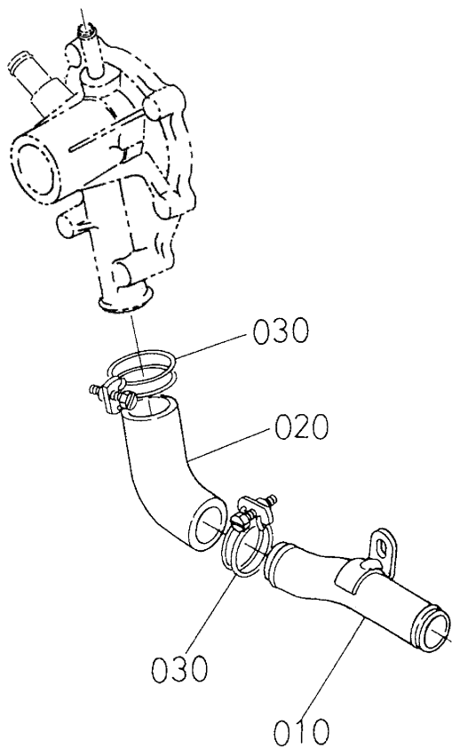
EG525-006-10
