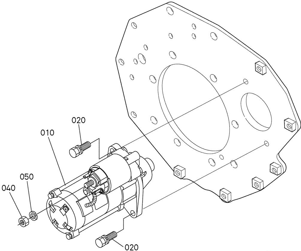
EG522-220-10
